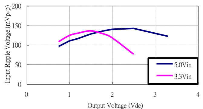
Figure 33: Input voltage ripple for various output models, I_O = 10 A ( C_{IN} = 4 \times 100 \mu F tantalum // 2 x 47 \mu F ceramic)
