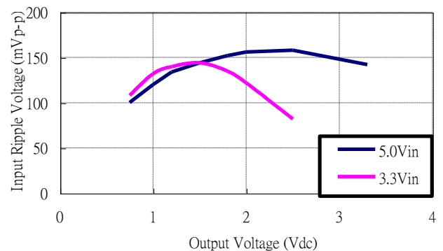
Figure 32: Input voltage ripple for various output models, I_O = 10 A ( C_{IN} = 2 \times 100 \mu F tantalum // 47 \mu F ceramic)
